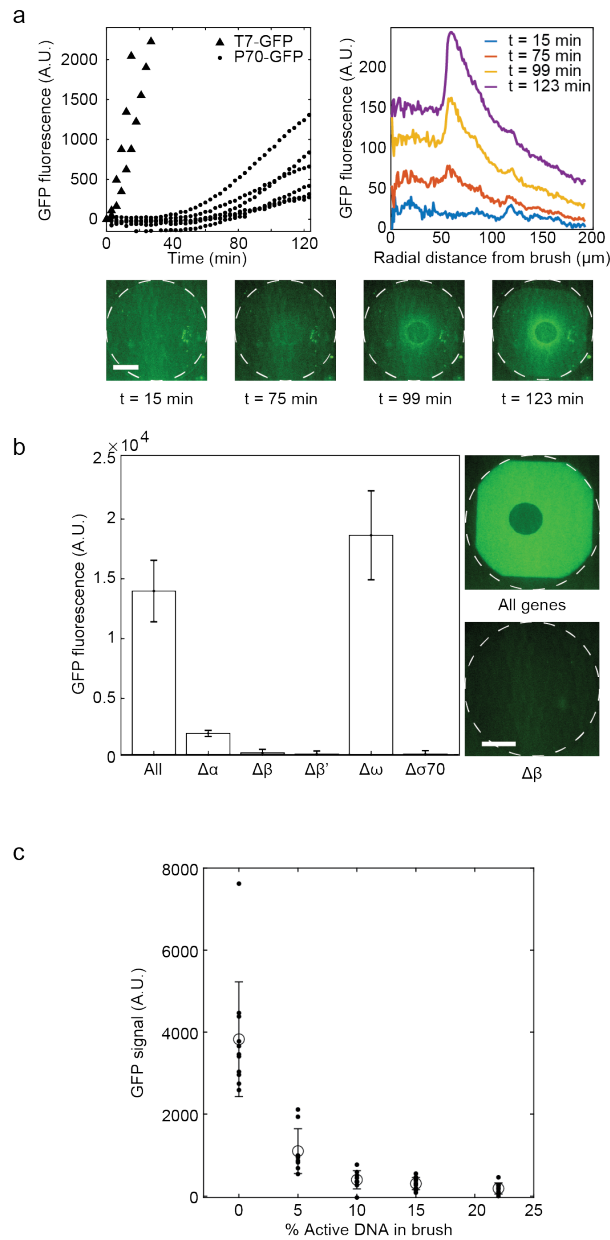
Supplementary Fig. 8. E. coli RNAP assembly and activity in 2D compartments. a , GFP expression dynamics in a 200 \mu\text{m} radius compartment (top left) either under T7 promoter (squares), or cascaded under P70 promoter, with RNAP genes under T7 promoter (circles). Fluorescent images (bottom) of P70-GFP in a representative compartment at different time points and the corresponding radial profiles (top right). Scale bar 100 \mu\text{m} . b , Deletion assay for RNAP genes in the brush and representative images. Scale bar 100 \mu\text{m} . c , Total signal of P70-GFP expressed by nascent RNAP in the presence of increasing fraction of active DNA in the brush. DNA brush content kept constant with passive DNA (Methods). Data are presented as mean and error bars represent \pm s.d. Detailed gene composition of all experiments shown in Supplementary Table 3. The number of samples for each data point ( a , b , c ) is listed in Supplementary Table 4.
