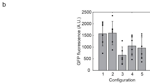
Supplementary Fig. 10. Spatial control of gene-expression. a , Scheme and representative images of 5 different configurations of DNA-brushes in a compartment. Each RNAP subunit gene brush (designated colors, top) at a fixed location, reporter P70-GFP (green) at variable locations. b , Total GFP signal in each of the five configurations. Data are presented as mean and error bars represent \pm s.d. Detailed gene composition of all experiments shown in Supplementary Table 3. The number of samples for each data point ( a , b ) is listed in Supplementary Table 4.
