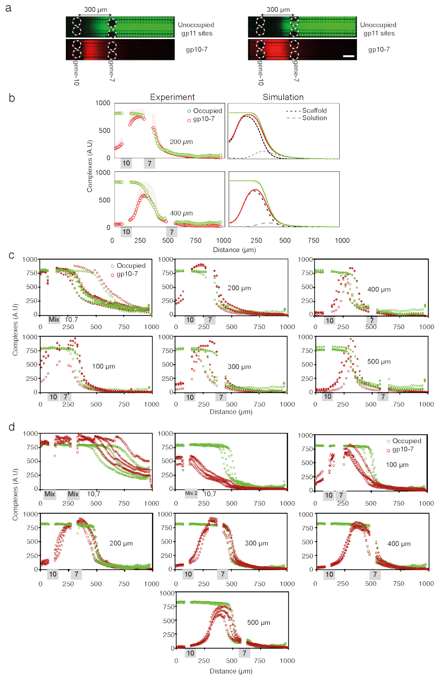
Supplementary Fig. 5. Synthesis and assembly of gp10-7 complexes in 1D layouts. a , two additional experiments similar to Fig. 2c with DNA brush doublets of gene-10 (left circles) and of gene-7 (right) patterned at a distance of 300 \mu\text{m} . Scale bar 100 \mu\text{m} . b , 1D profiles of gp10-7 complexes with genes in separate DNA brushes, 200 \mu\text{m} (top) or 400 \mu\text{m} (bottom) apart. Data are presented as the mean, error bars are +s.d. Simulation of scaffolded and solution assembly profiles at the designated distance. Integrated signal shown in Fig. 2e. c , All the 1D profiles averaged in Fig. 2d. d , 1D profiles of gp10-7 complexes of an additional set of experiments at conditions slightly different than of c . Detailed gene composition of all experiments shown in Supplementary Table 3. The number of samples for each data point ( a , b , c , d ) is listed in Supplementary Table 4.
