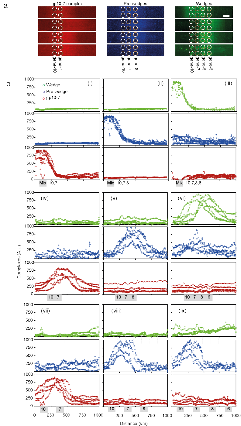
Supplementary Fig. 6. 1D profiles of T4 wedge assembly. a , Images of four compartments, part of the experiments in Fig. 3a. Designated genes and distances as in Fig. 3a. Scale bar 100 \mu\text{m} . b , All 1D profiles averaged in Fig. 3b. Profiles are of gp10-7 complex (red), pre-wedges (blue) and wedges (green) for mixed (i, ii, iii) separated (iv, v, vi) and spread-out (vii, viii, ix) layouts. Detailed gene composition of all experiments shown in Supplementary Table 3. The number of samples for each data point ( a , b ) is listed in Supplementary Table 4.
