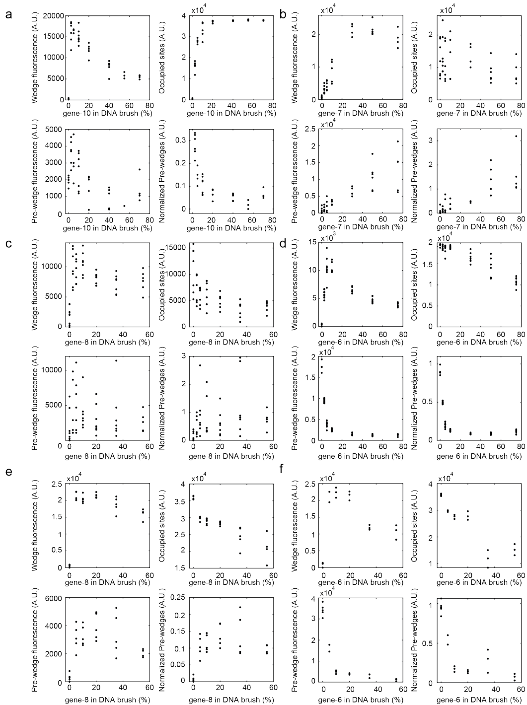
Supplementary Fig. 3. On-chip wedge assembly as a function of gene fraction. Dose response curves of total wedges (FL-gp53), occupied sites (complement of FL-gp10), pre-wedges (FL-gp6) and pre-wedges normalized by number of occupied sites, all at different gene fractions (all wedge proteins other than the designated kept constant). a-d , Individual data points of Fig. 1e. Dose response for gene-10 (a), gene-7 (b), gene-8 (c), gene-6 (d). e, f , Additional dose response experiments for gene-8 (e) and gene-6 (f), carried out in different conditions than c, d . Gene compositions of all experiments shown in Supplementary Table 3. The number of samples for each data point ( a-f ) is listed in Supplementary Table 4.
