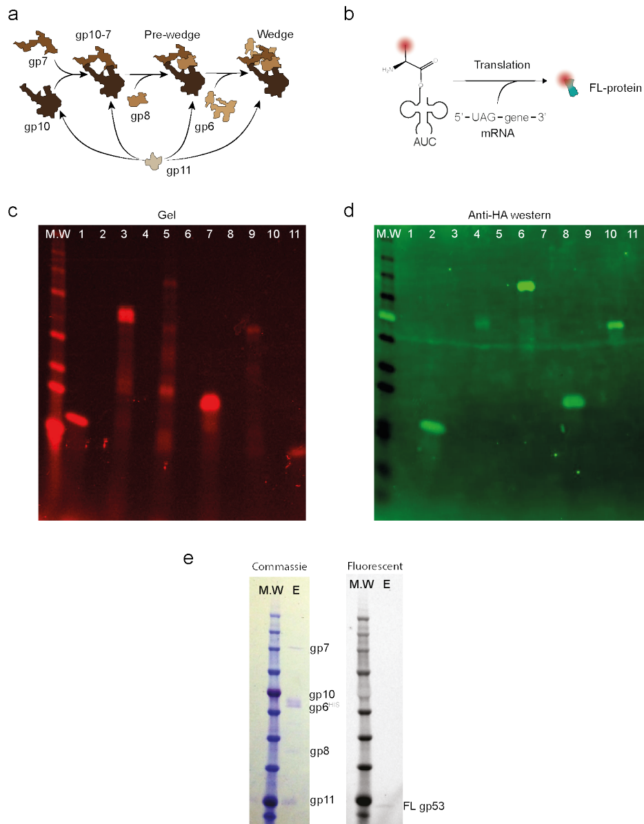
Supplementary Fig. 2. T4 wedge assembly line and tagging of wedge proteins in off-chip cell-free expression (CFE) reactions. a , T4 wedge assembly line, gp11 is the only protein that binds non-sequentially. Wedge proteins 6, 7, 8, 10, and 11 bind in a 2:1:2:3:3 stoichiometry. Adapted from 27,28 . b , Scheme, site-specific incorporation of FL unnatural amino acid. Supplementing the CFE reaction with a gene coding for the AUG stop codon, as the second amino acid, and with tRNA of the anti-codon AUC, charged with FL unnatural amino acid, results in a FL-protein. c , d , N-terminus FL or C-terminus HA tag variants of wedge proteins separately expressed in solution and resolved by 4-20% gradient denaturing PAGE. (1) FL-gp11, (2) gp11 HA, (3) FL-gp10, (4) gp10 HA, (5) FL-gp7, (6) gp7 HA, (7) FL-gp8, (8) gp8 HA, (9) FL-gp6, (10) gp6 HA, and FL-gp53. c , A fluorescent scan of the gel. d , Anti-HA western blot of the gel using ATTO488 labeled antibodies (Methods). e , CFE reaction of gp11:gp10; gp7; gp8; gp6 HIS and FL-gp53 purified using Ni 2+ agarose and resolved by SDS-PAGE (Methods). Fluorescent scan of the gel and commassie staining of all proteins part of the purified complex.
