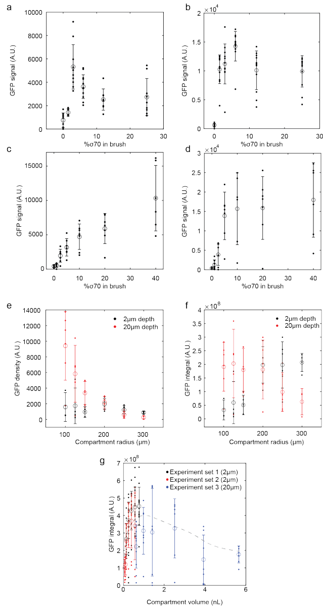
Supplementary Fig. 9. Effect of compartment dimensions on GFP expression. a-c , Individual data points and means of \sigma 70 gene dose response of shown in Fig. 5b, at 2 \mu\text{m} ( a , c ) and 20 \mu\text{m} ( b ). Core RNAP expressed from gene brushes ( a , b ) or added in purified form to the solution ( c ). d , Additional set of experiments as in c , showing similar results. e , GFP signal density and f , integrated GFP signal over the entire compartment as a function of compartment radius. Data correspond to Fig. 5c. g , Individual data points and mean of the integral of HA-GFP signal over entire compartment surface, at variable compartment radii and depth, shown in Fig. 5c. Data was collected from 3 different sets of experiments containing compartments with radii varying from 100 \mu\text{m} to 300 \mu\text{m} . The compartments in experiment set 1 and 2 were 2 \mu\text{m} deep, and the compartments in experiment set 3 were 20 \mu\text{m} deep. Line is a guide to the eye. Data are presented as mean and error bars represent \pm s.d. Detailed gene composition of all experiments shown in Supplementary Table 3. The number of samples for each data point ( a , b , c , d , e , f , g ) is listed in Supplementary Table 4.
