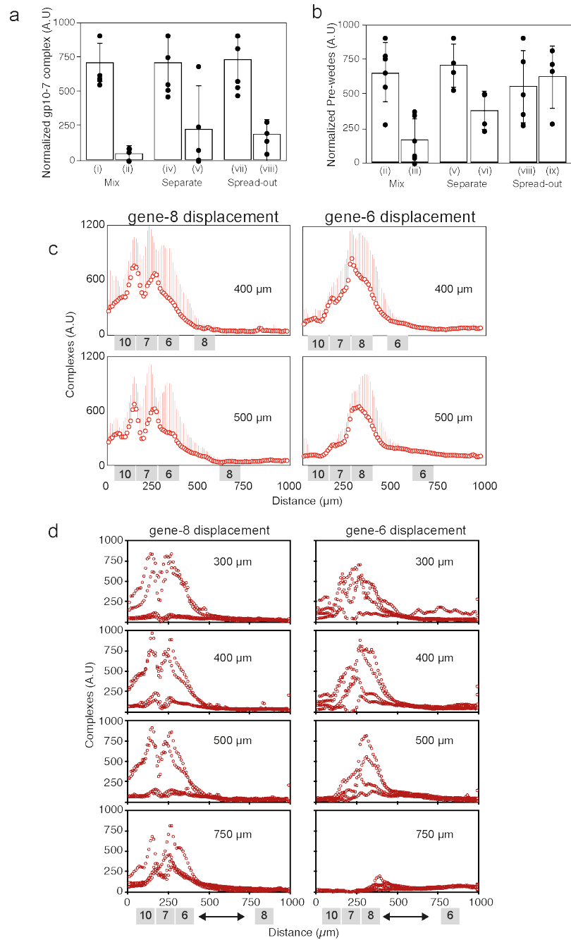
Supplementary Fig. 7. Effect of brush layout on assembly yield. a , Normalized total gp10-7 complexes (Supplementary Fig. 6b, red curves) formed in the absence and presence of gene-8 (layouts (i), (iv), (vii), and (ii), (v), (viii), respectively). b , Normalized total pre-wedges (Supplementary Fig. 6b, blue curves) formed in the absence and presence of gene-6 (layouts (ii), (v), (viii), and (iii), (vi), (ix), respectively). In a and b the mean value is shown and error bars representing \pm s.d. Normalization methodology is described in Methods. c , The effect of gene-8 and gene-6 displacement on wedge formation, showing 400 \mu\text{m} (top) and 500 \mu\text{m} (bottom) displacement. Integrated signal shown in Fig. 3e. d , Individual data points of 1D profiles that appear in Fig. 3d and in c. Data ( c , d ) are presented as mean and error bars are \pm s.d. Detailed gene composition of all experiments shown in Supplementary Table 3. The number of samples for each data point ( a , b , c , d ) is listed in Supplementary Table 4.
