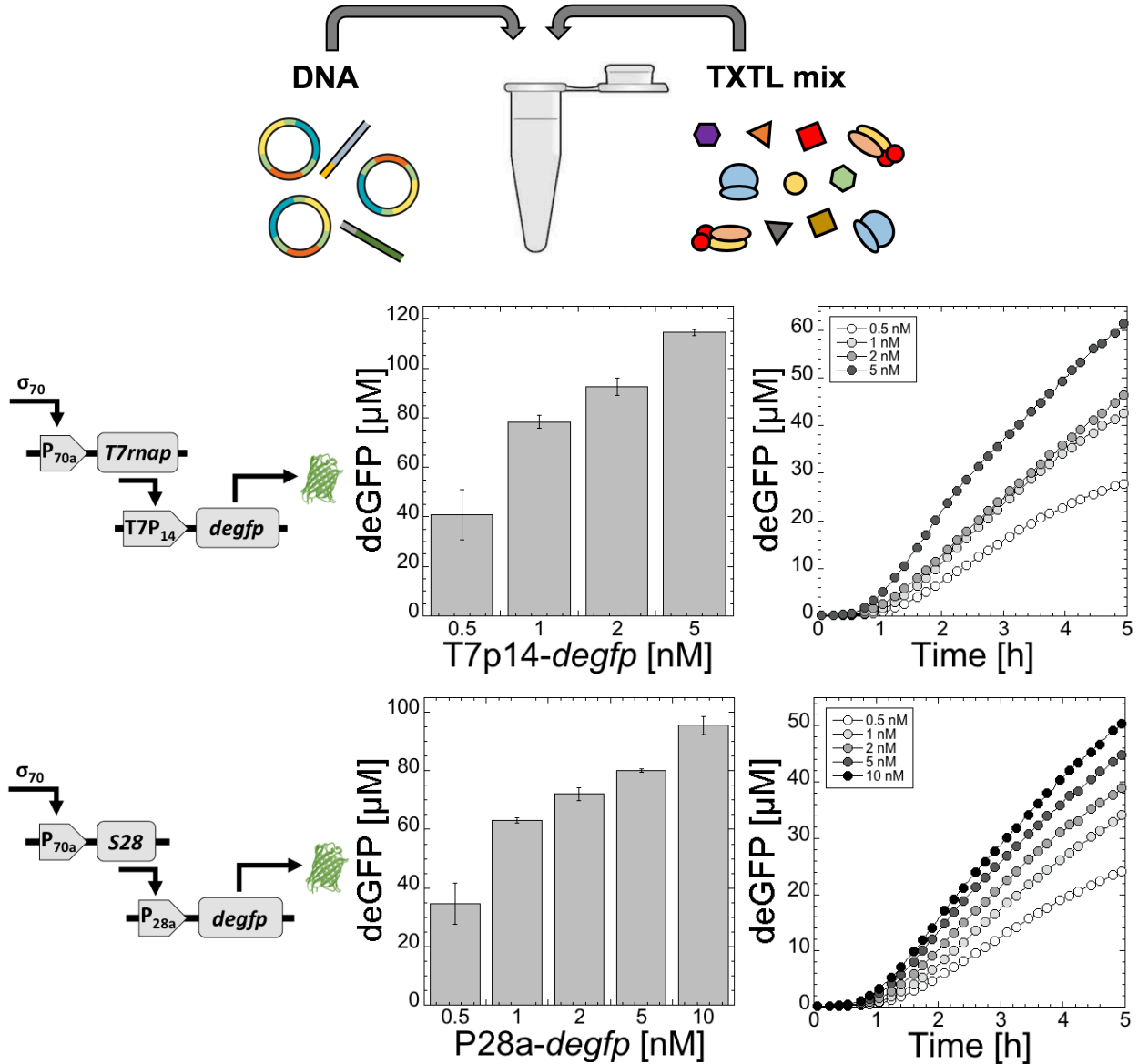
Figure S2. Batch mode TXTL reactions using transcriptional activation cascades. Top. the reaction is assembled in teste tube reactions (10 \mu l) or on well plates (2 \mu l). Middle row. using a T7 cascade (P70a-T7map fixed at 0.2 nM), one can produce up to 115-120 \mu M deGFP, which corresponds to 3 mg/ml of proteins. Bottom row. with a S28 cascade (P70a-S28 fixed at 0.5 nM), one can get up to 90-100 \mu M deGFP, which corresponds to a maximum or 2.5 mg/ml or protein. The kinetics is shown for the first 5 hours at different concentration of the reporter plasmid. When mreB is expressed using the S28 cascade, more than 90% of the liposomes acquire their final shapes after 5 hours.
