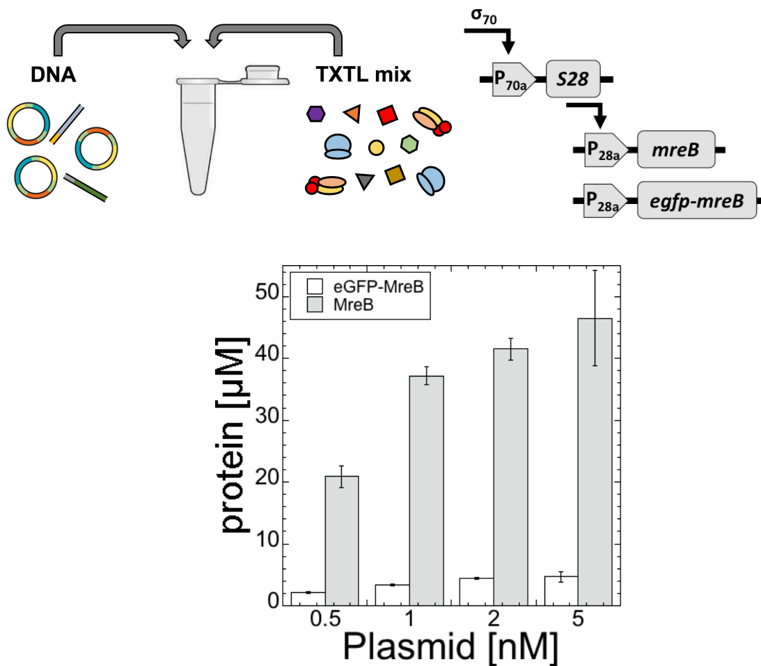
Figure S3. Batch mode TXTL reactions using the S28 transcriptional activation cascade for synthesizing MreB and eGFP-MreB. Top. The reaction is assembled in test tube reactions (10 \mu l) or on well plates (2 \mu l). Bottom. P70a-S28 is fixed at 0.5 nM. Four combinations of the two other plasmids were tested in which the concentration of P28a- egfp-mreB is 10 times smaller than P28a- mreB : 0.5, 1, 2 and 5 nM P28a- mreB (0.05, 0.1, 0.2 and 0.5 nM P28a- egfp-mreB ). The endpoint concentration of eGFP-MreB was measured by fluorescence, the concentration of unlabeled MreB was estimated based on the S28 cascade quantification shown in Fig. S2 (using deGFP).
