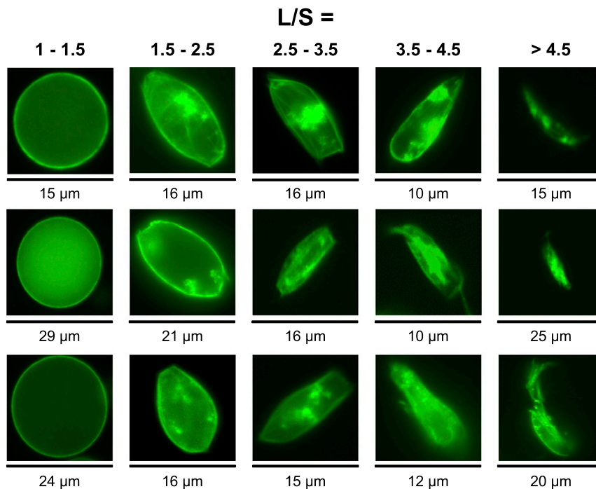
Fig. 4. Sample fluorescence images of liposomes for different L/S ratios. The images were all shot with a 40 \times objective.
