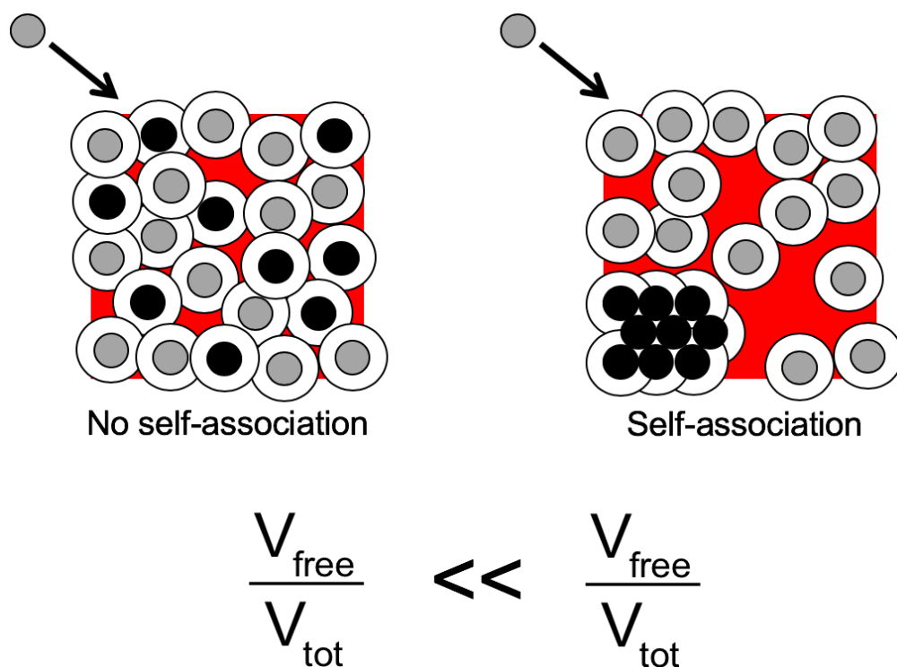
Figure S10. Schematic of the effect of molecular crowding on the excluded volume. This figure is inspired from (1, 2). The excluded volume decreases when a species of molecule (dark bullet) self-associate in the presence of other macromolecules (grey bullets), providing more space to add another molecule. The white ring around each molecule represent the excluded volume. As a consequence of the excluded volume in crowded media, reactions that increase available volume are favored by crowding conditions. These processes include the association of molecules as shown in this figure.
